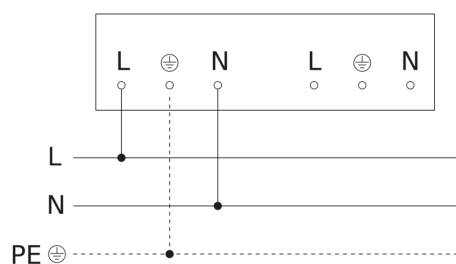
Circuit diagram 1
